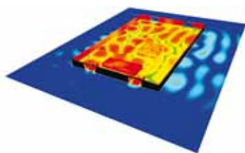
1U server emissions at 3GHz (seam leakage)
